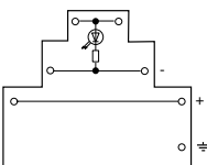
AB1 ET3235UTLM (R = 2.2 k, 0.35 Вт)
